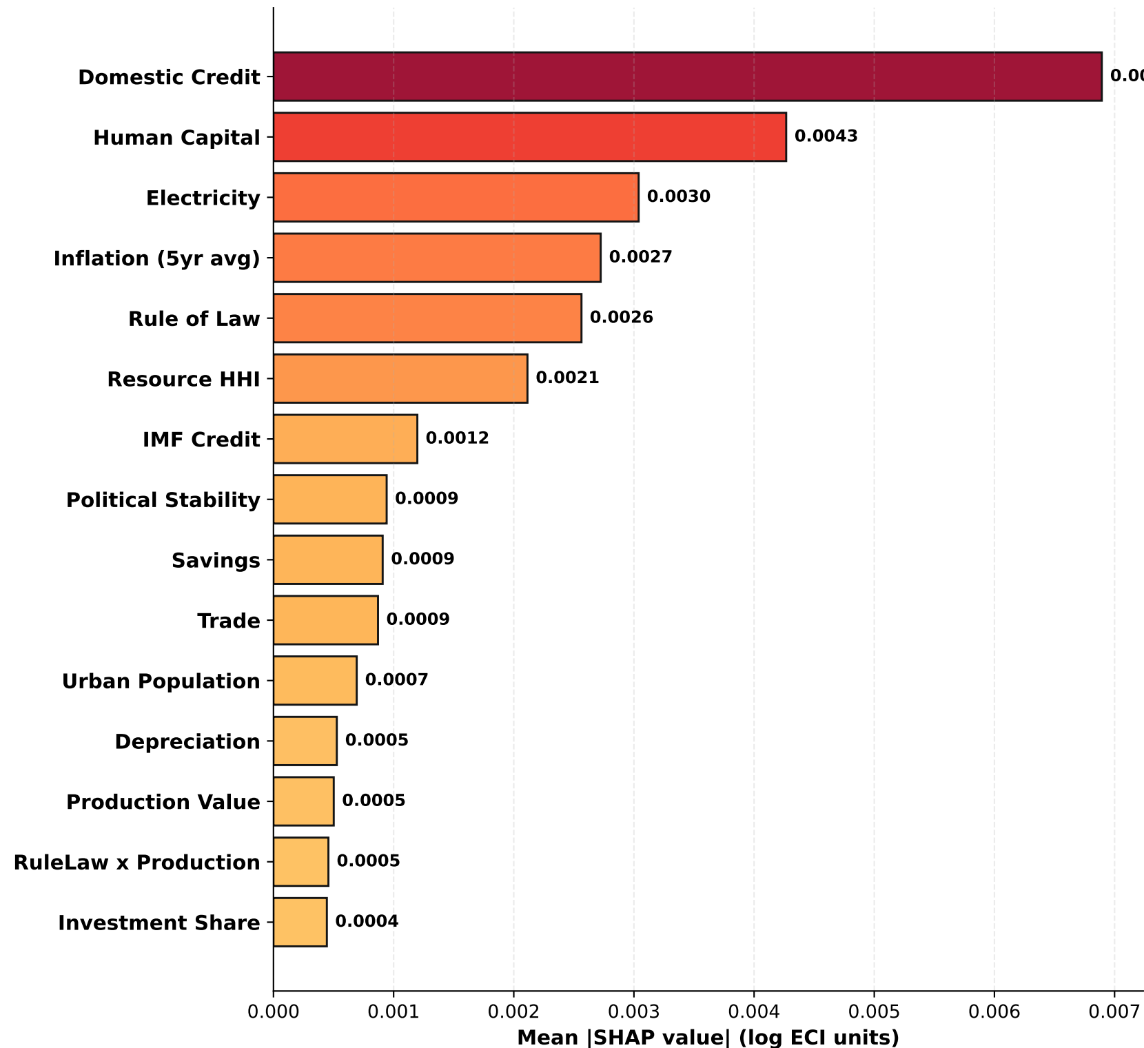
SHAP — Random Forest Test set, top 15 features (L1_ECI excluded)
