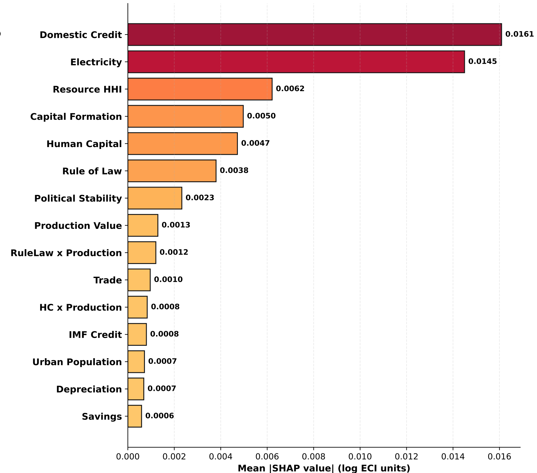
SHAP — XGBoost Test set, top 15 features (L1_ECI excluded)
